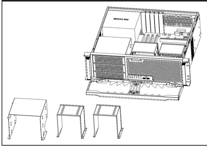
3 x 5.25" ODD and 5 x 3.5" and 2 x 2.5" HDD搭載可能
